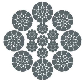
8×K26WS-IWRC(7x19S)
