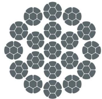
18xK7-WSC
