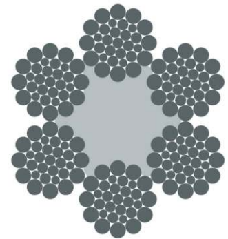
6×31WS-FC
