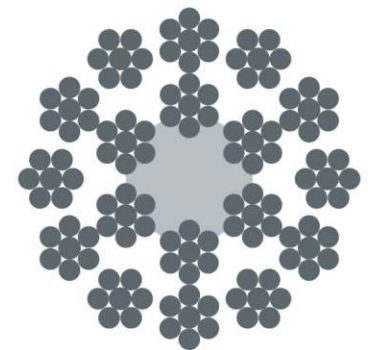
18×7-FC
