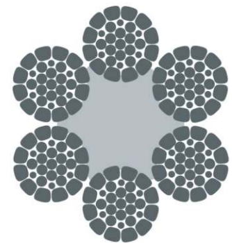
6×K31WS-FC
