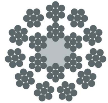
17×7-FC
