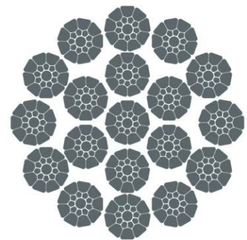
18xK19S-FC
