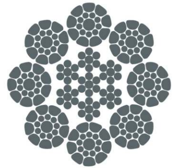
8×K19S-IWRC(7x7)
