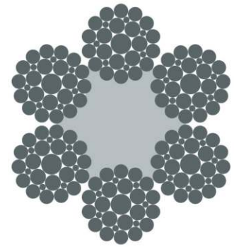
6×29F-FC
