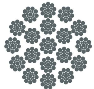
18×19S-WSC
