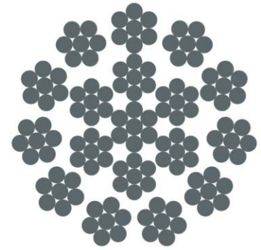
17×7-WSC
